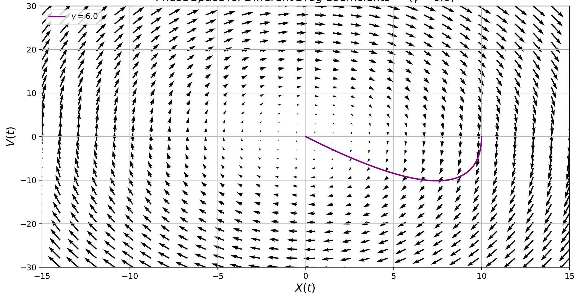
Phase Space for Different Drag Coefficients – ( \gamma = 6.0 )
